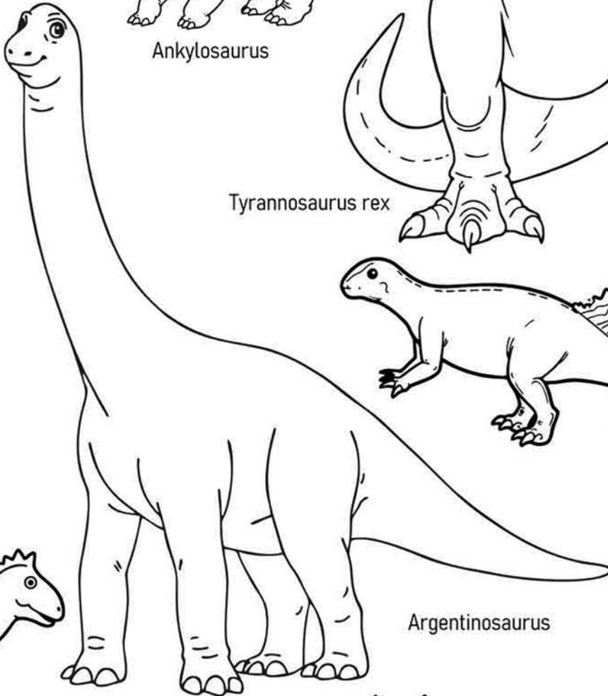
Psittacosaurus
